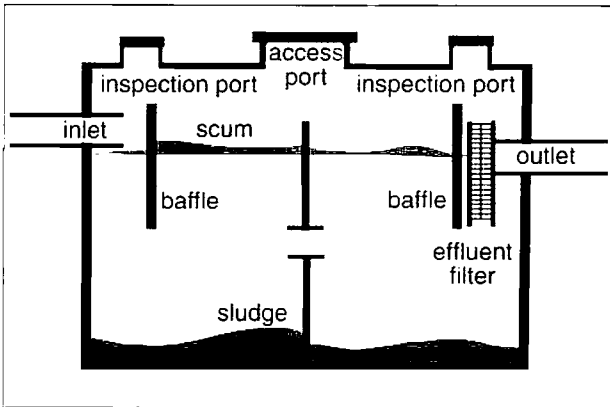
Cross-section of a two-compartment septic tank
